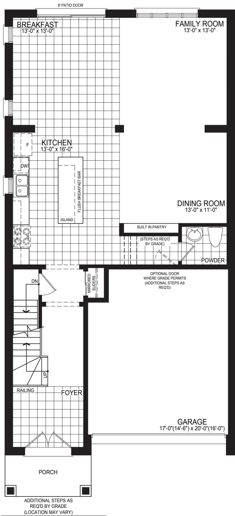
MAIN FLOOR PLAN STYLE B
