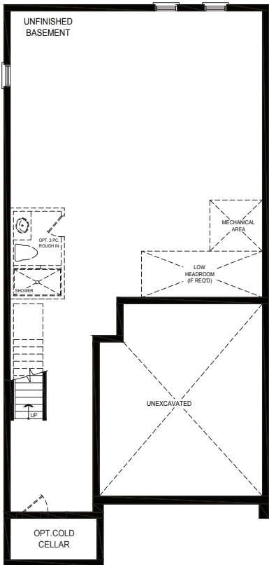
BASEMENT PLAN STYLE B
