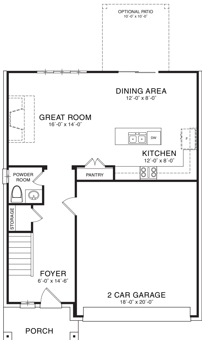
MAIN FLOOR PLAN STYLE D
