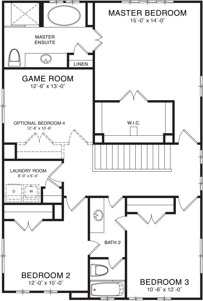
SECOND FLOOR PLAN STYLE D
